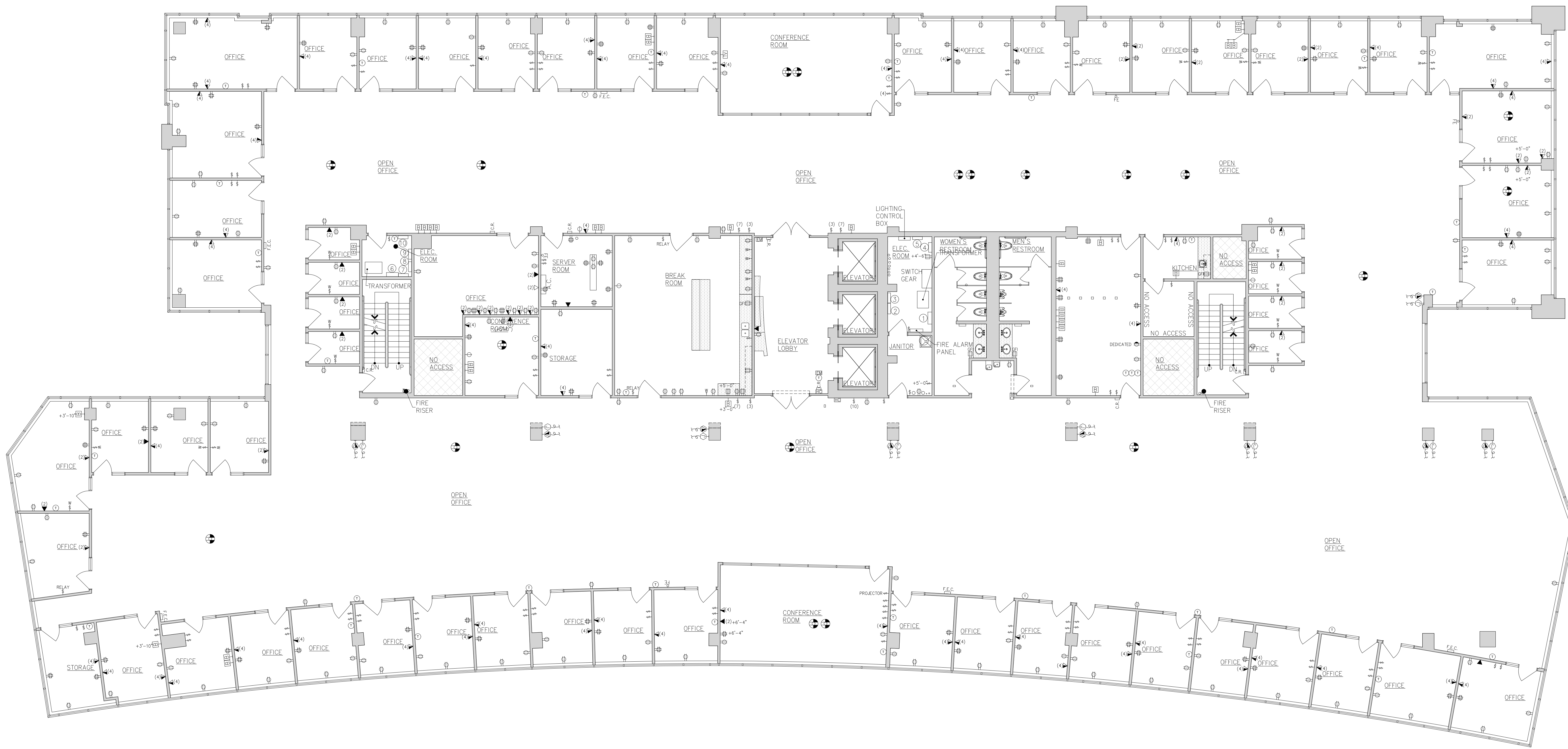
THIRD FLOOR POWER AND SIGNAL PLAN 1
